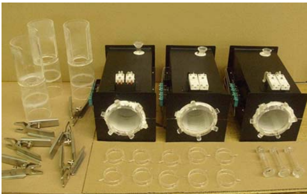
Figure 3.14. New equipment for the ^{131}\text{I} production area
